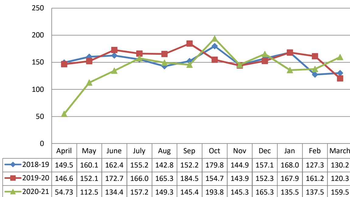
Graph 3.4: Graphical presentation of General Index in last three years 2018-19, 2019-20 & 2020-21
